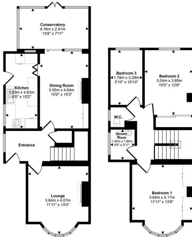
Ground Floor Approx 58 sq m / 626 sq ft
